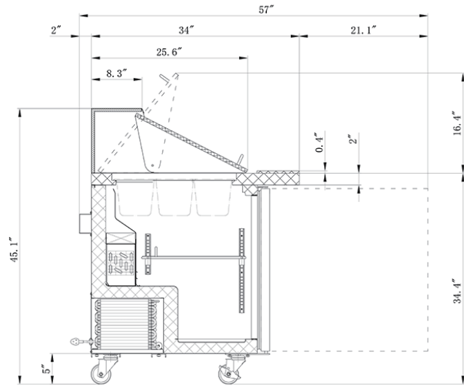
SECTION VIEW
