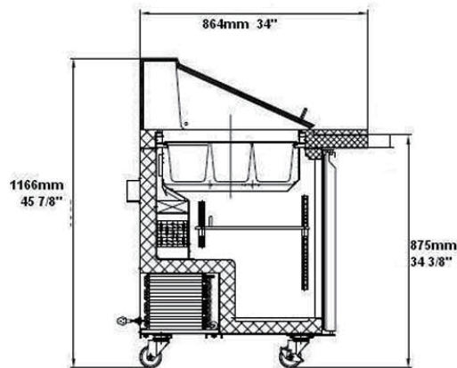
Section View
