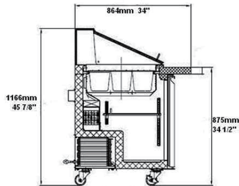
Section View
