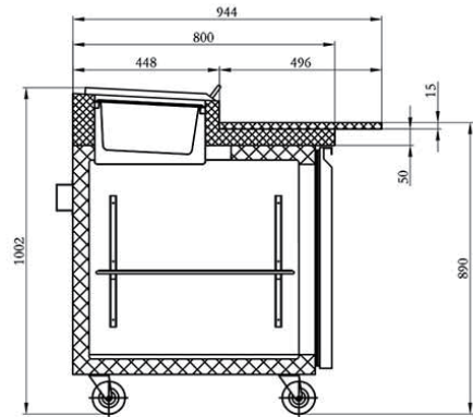
SECTION VIEW
