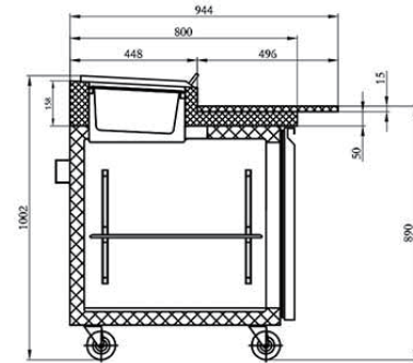
SECTION VIEW
