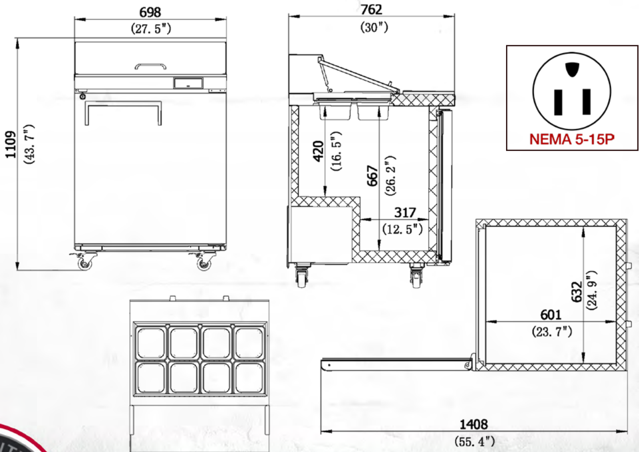
PRODUCT DRAWINGS
