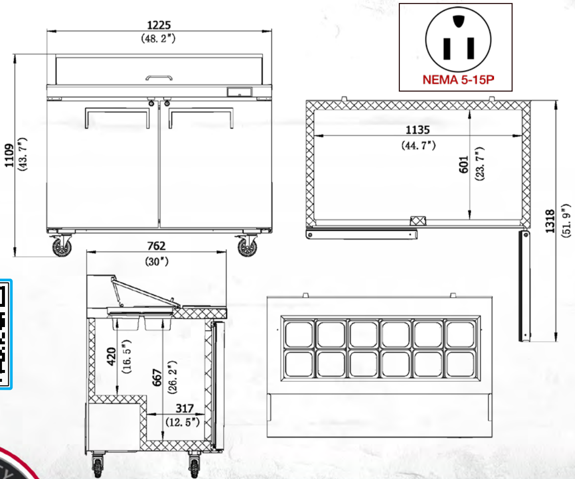
PRODUCT DRAWINGS
