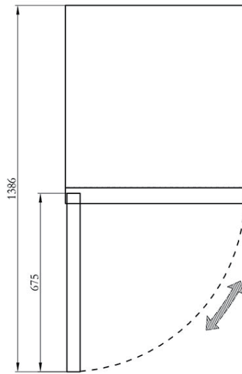
PLAN
