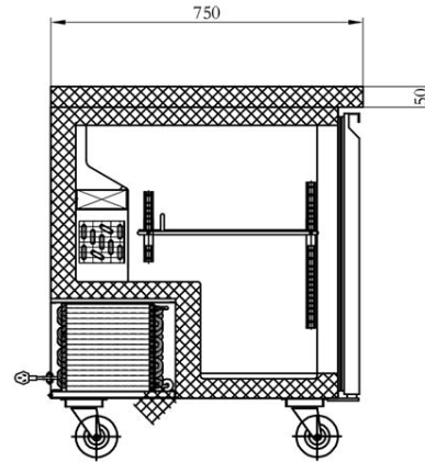
SECTION VIEW
