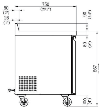
SECTION VIEW
