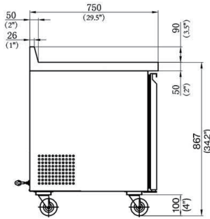
SECTION VIEW
