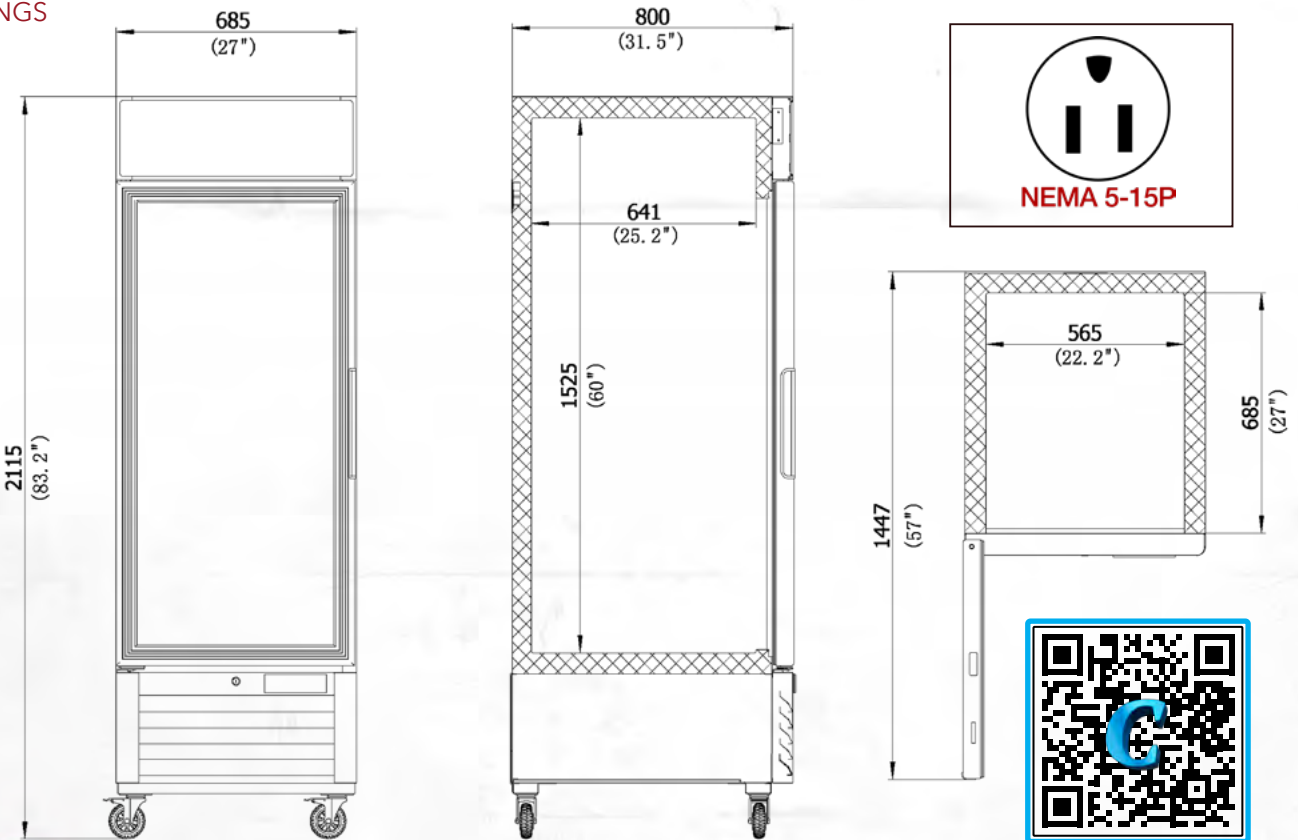
PRODUCT DRAWINGS
