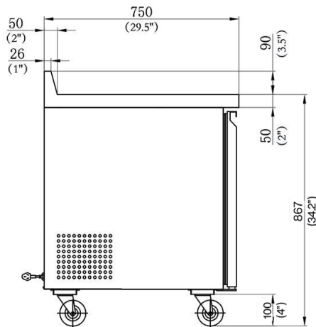
SECTION VIEW
