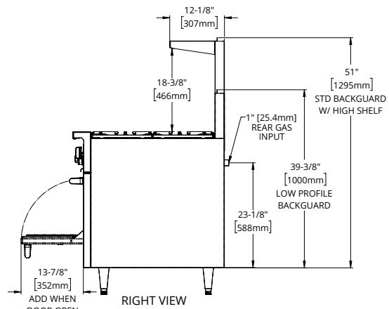
RIGHT VIEW
