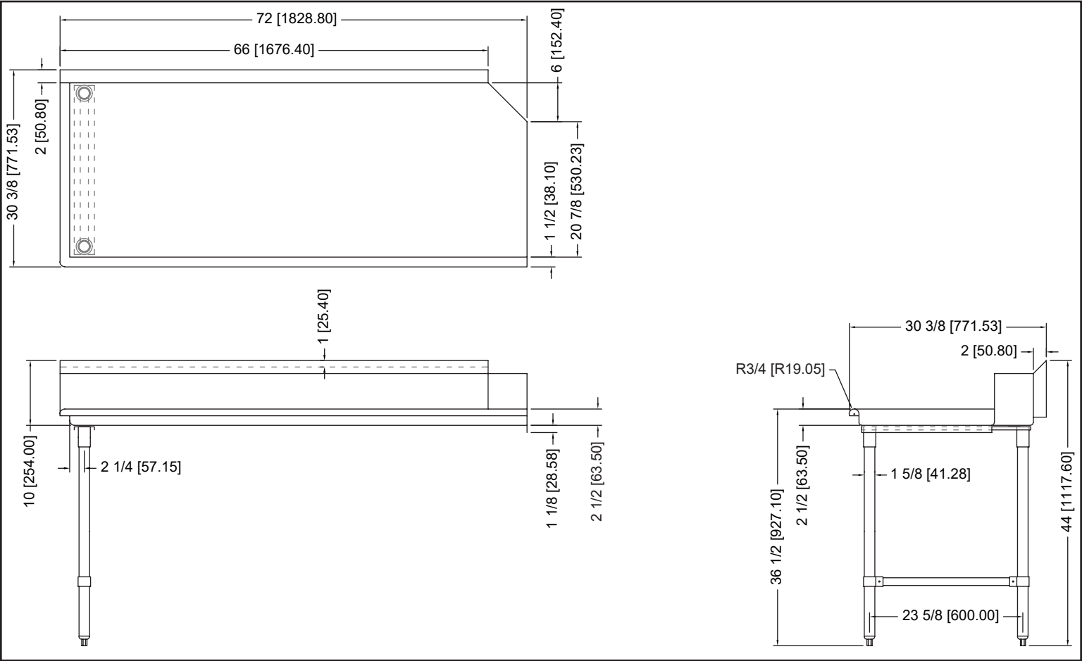
47746 - 72" SOILED DISH TABLE WITH SINK - RIGHT SIDE
