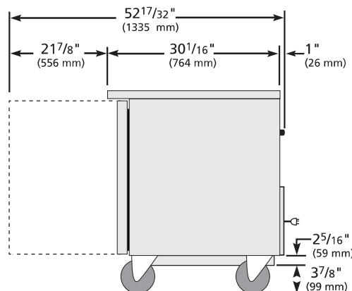
RIGHT VIEW
