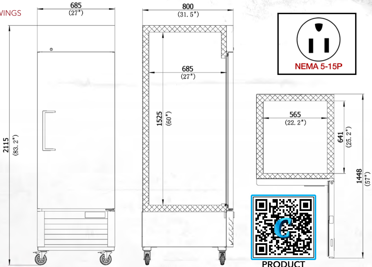
PRODUCT DRAWINGS
