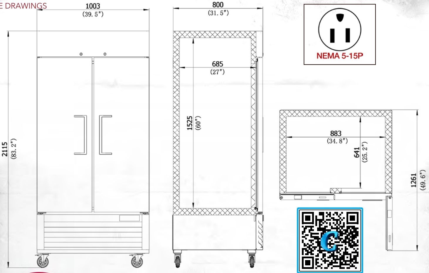
PRODUCT DRAWINGS
