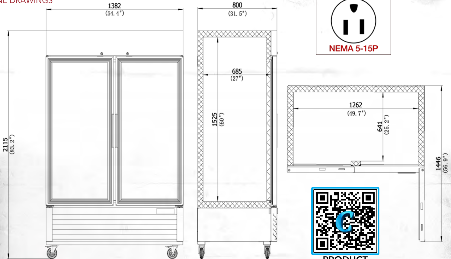
PRODUCT DRAWINGS
