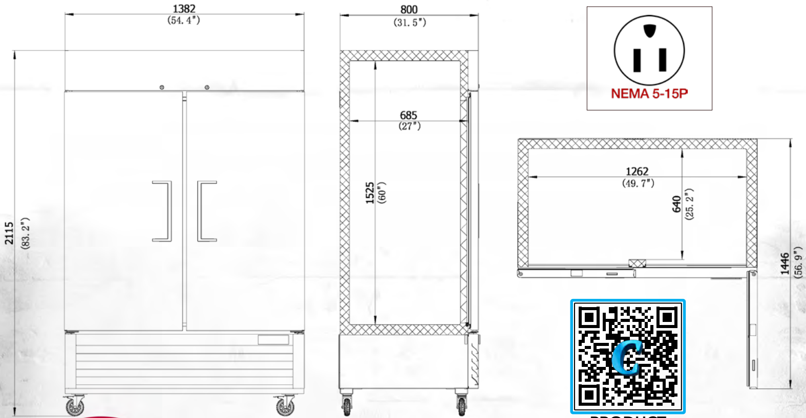
PRODUCT DRAWINGS
