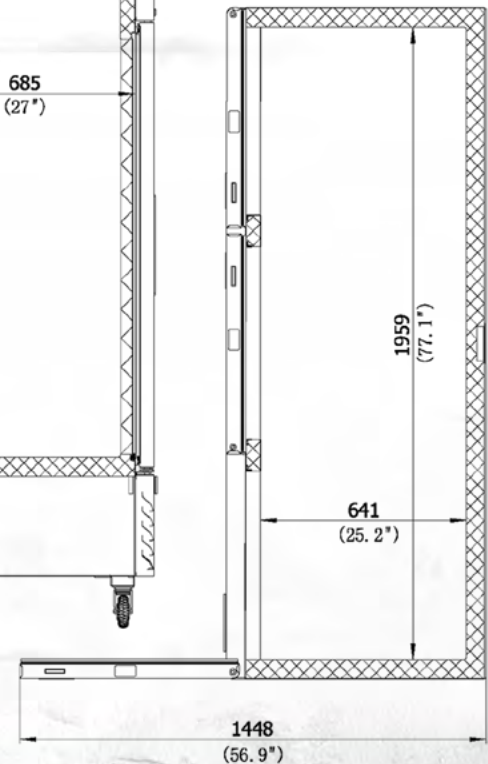
PRODUCT DRAWINGS
