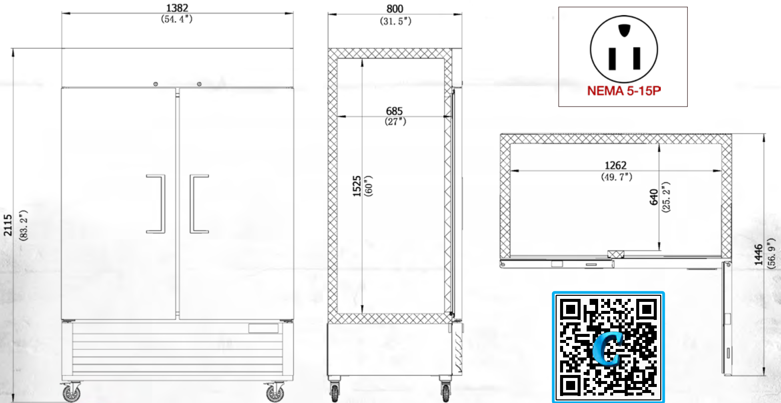
PRODUCT DRAWINGS
