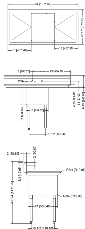
ONE TUB SINK WITH TWO DRAIN BOARD
