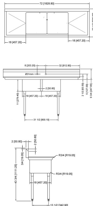
TWO TUB SINK WITH TWO DRAIN BOARD
